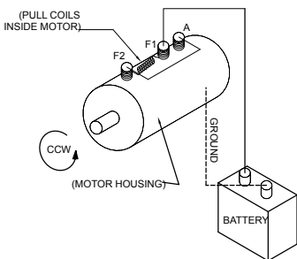
FIGURE 2 MOTOR-COUNTER-CLOCKWISE ROTATION
