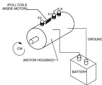
FIGURE 1 MOTOR-CLOCKWISE ROTATION
