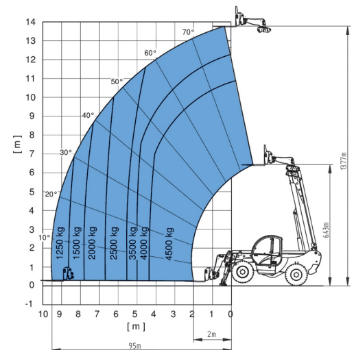
Lift capacity chart (with stabilisers)
